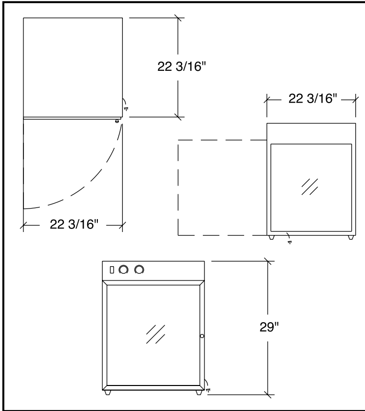
Model HDC-4, Heated Display Cabinet
